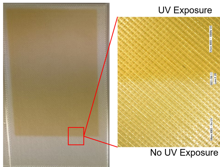
Figure 11. ULTEM™ 9085 resin plaque with rectangular area that was exposed to UV. The ULTEM™ 9085 resin material appears to have darkened and yellowed from the UV exposure.
